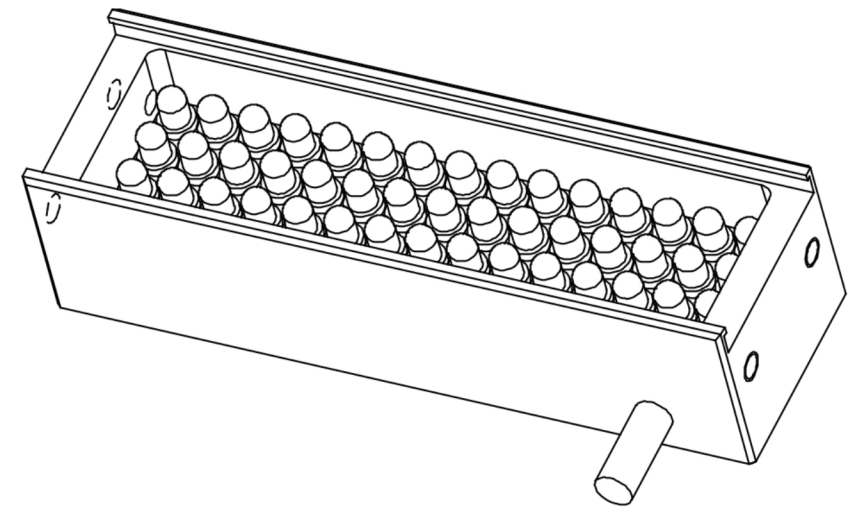
Details of Connector
